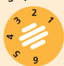
Output ▲ (evening)
